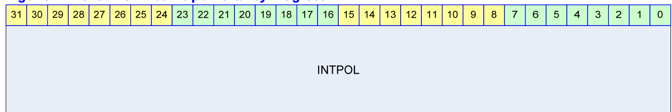
Figure 24-9 GPIO Interrupt Polarity Register
