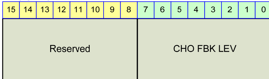
Figure 23-58 CHO (7) Register
