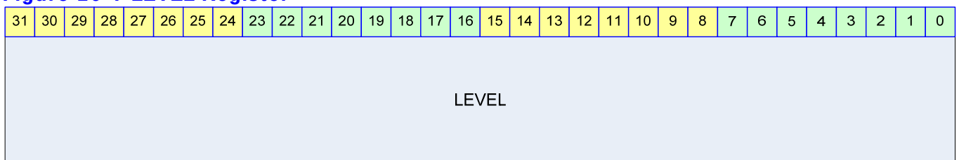
Figure 10-7 LEVEL Register
