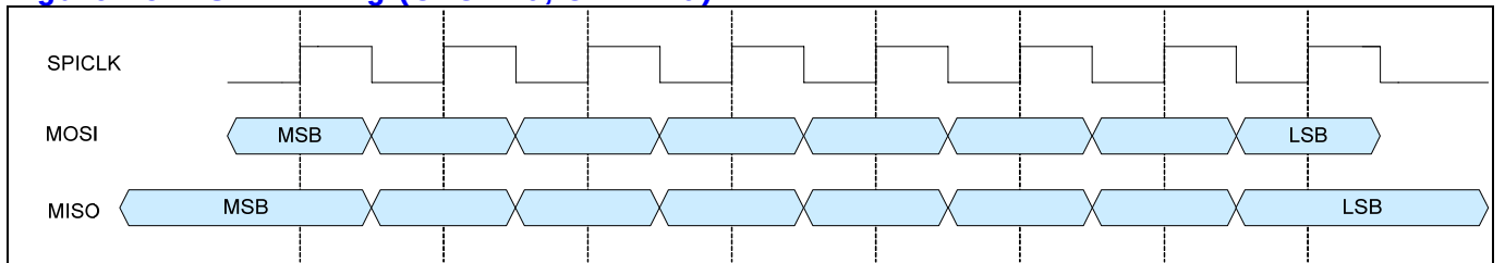
Figure 25-2 SPI Timing (CPOL=0, CPHA=0)
