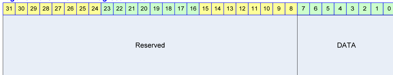
Figure 16-5 I2CDAT Register Bits
