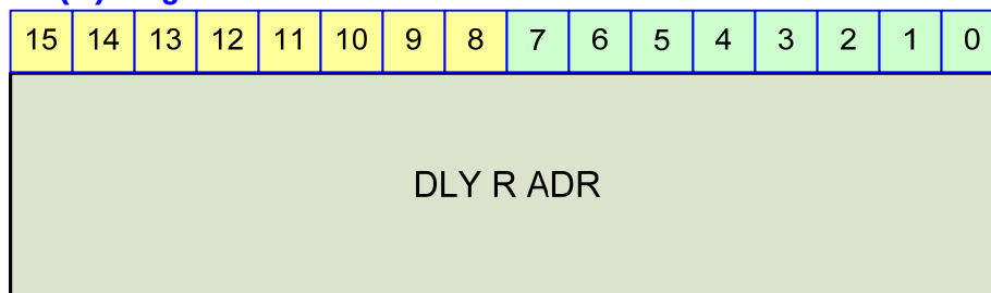
Figure 23-98 ADR(5) Register
