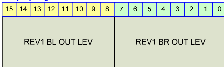
Figure 23-79 REV1(11) Register
