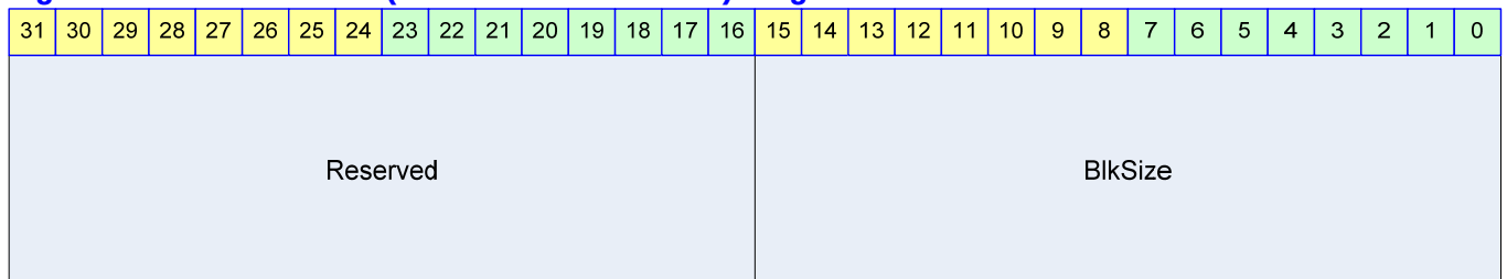
Figure 27-12 SDBSIZE (MMC/SD Block Size) Register Bits
