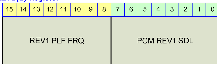
Figure 23-70 REV1(2) Register
