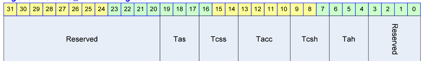
Figure 7-3 SMC_BANKx Register
