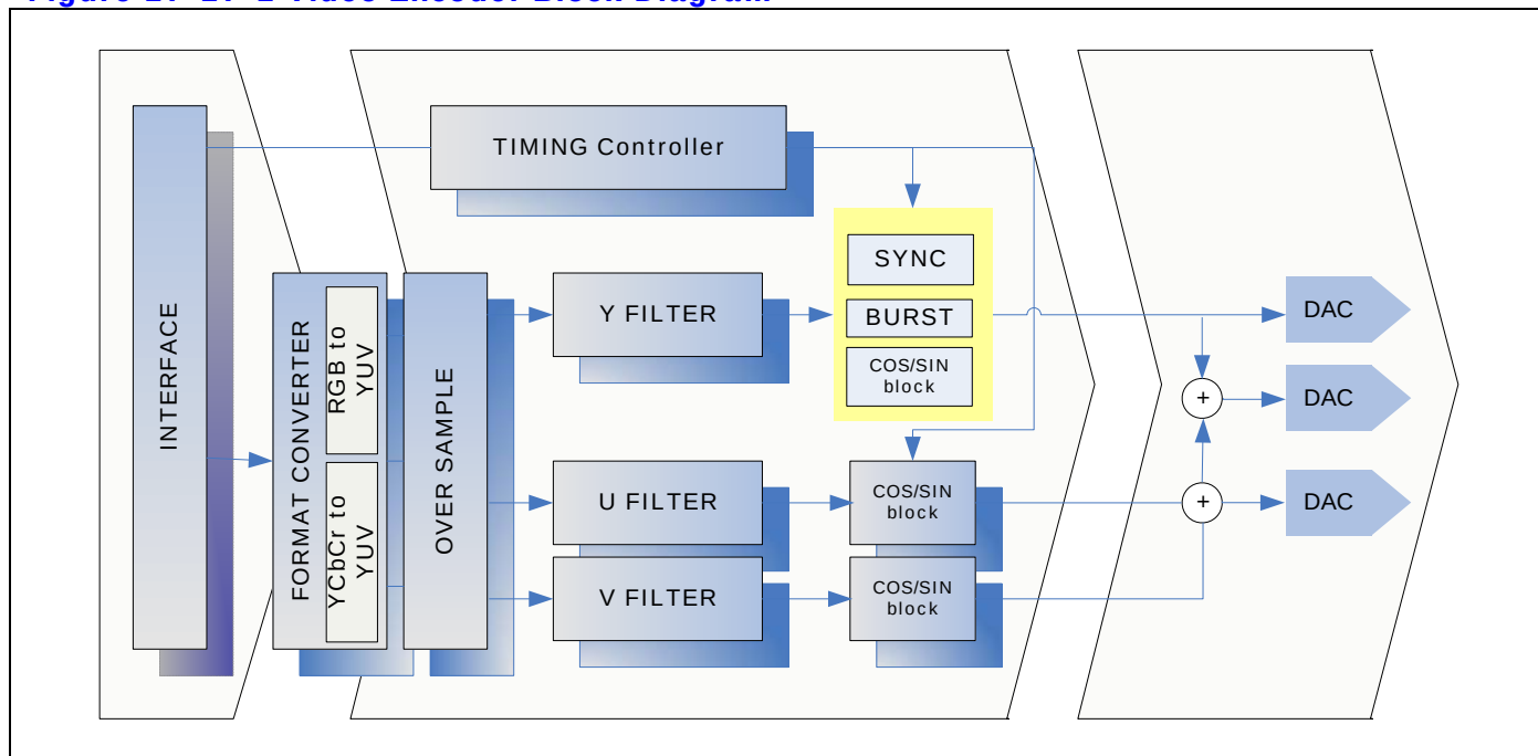
Figure 17-17-1 Video Encoder Block Diagram
