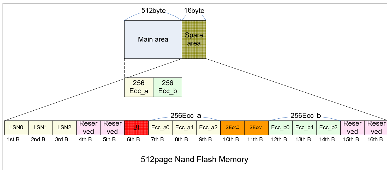
Figure 9-19 Spare area
