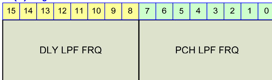
Figure 23-65 DLY(1) Register
