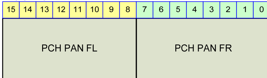
Figure 23-64 PCH(6) Register
