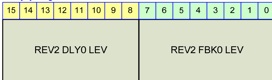
Figure 23-82 REV2(3) Register
