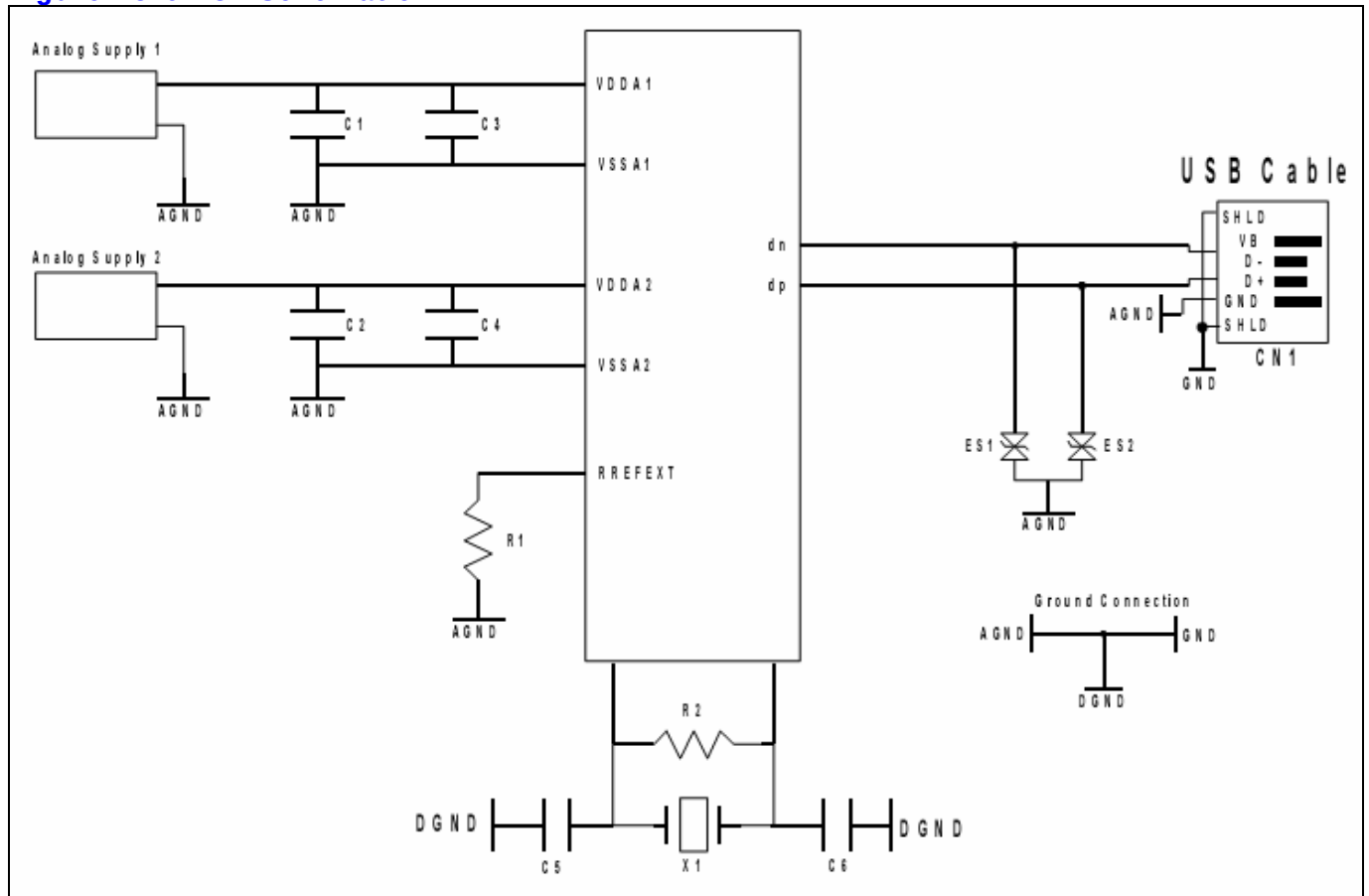
Figure 28-6 PCB Schematic
