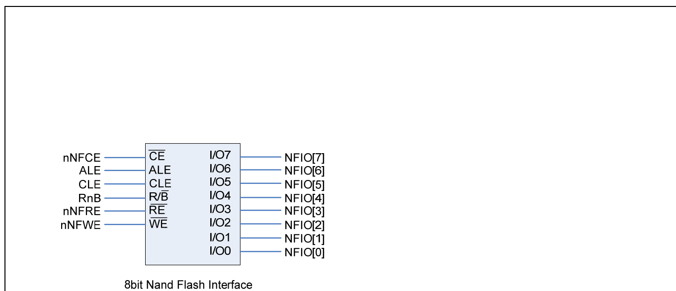
Figure 9-5 Interface example
