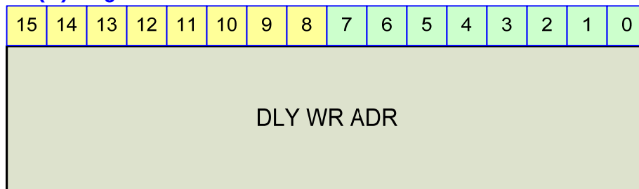
Figure 23-97 ADR(4) Register
