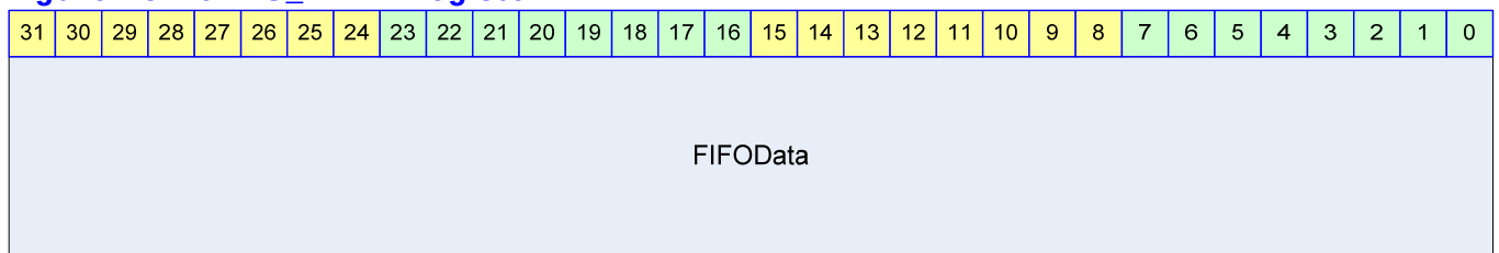
Figure 15-10 I2S_DATA Register
