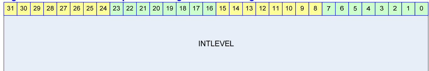
Figure 24-8 GPIO Interrupt Level/Edge Selection Register
