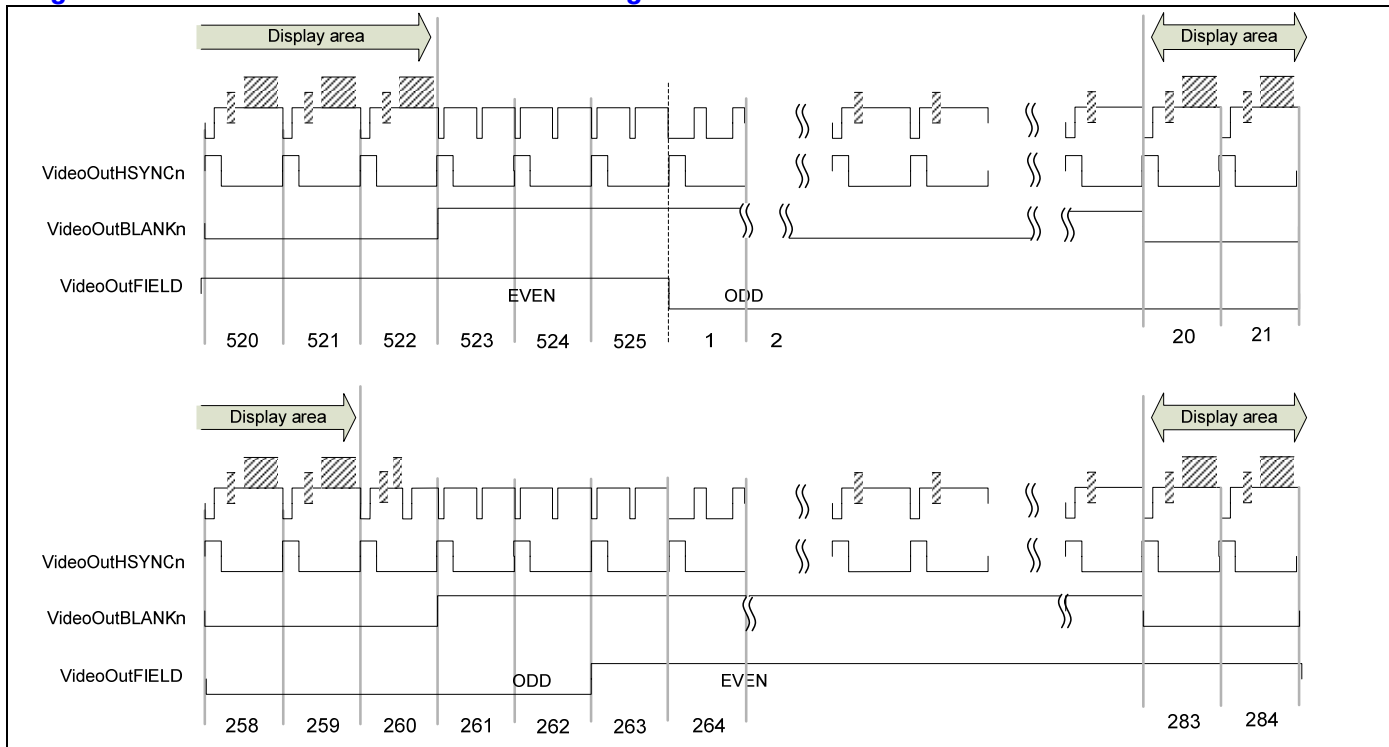
Figure 17-17-6 BT656 NTSC mode Timing
