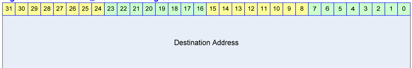
Figure 12-6 DMA2D_DSTADDR Register
